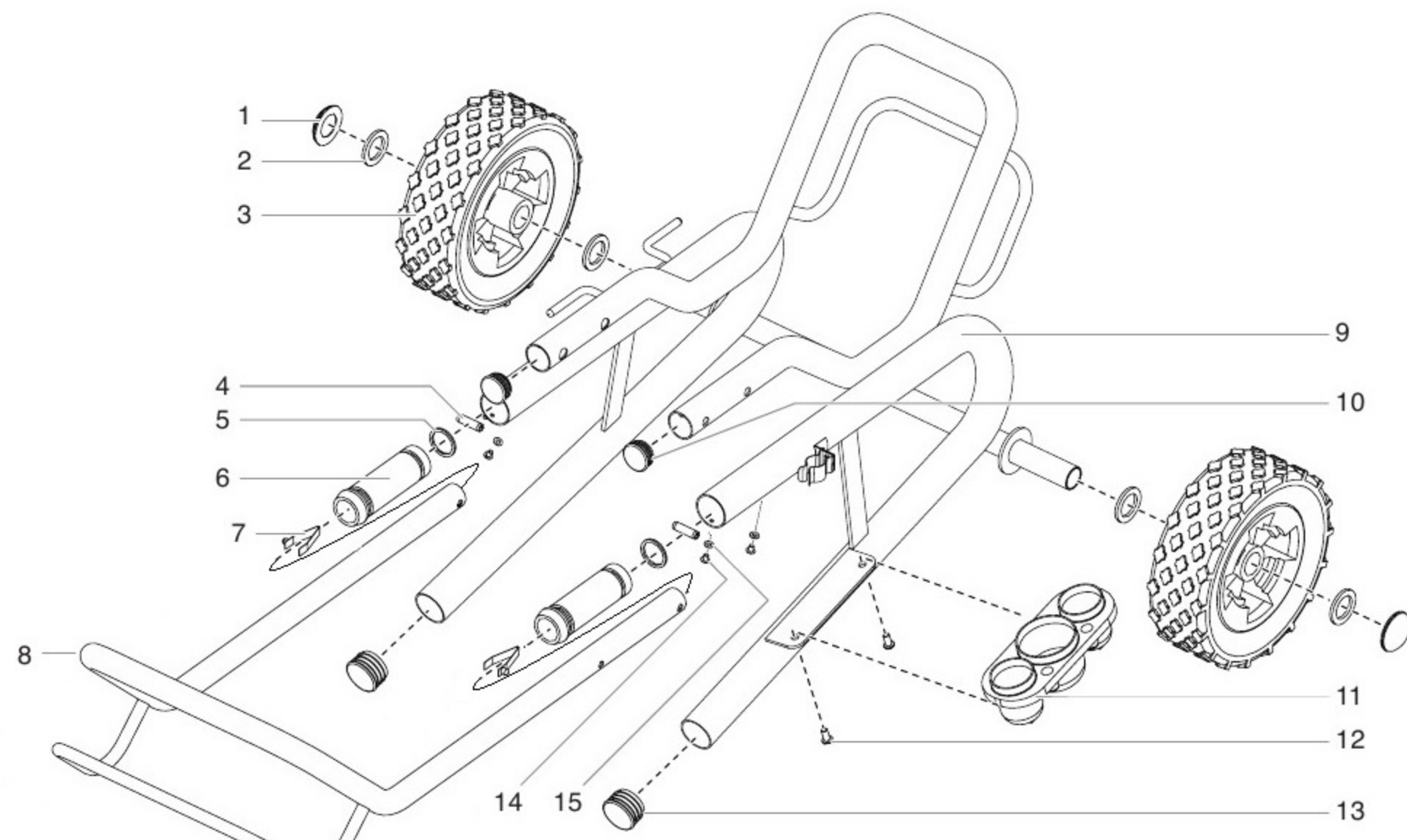
Low rider Assembly (P/N 0558392)
